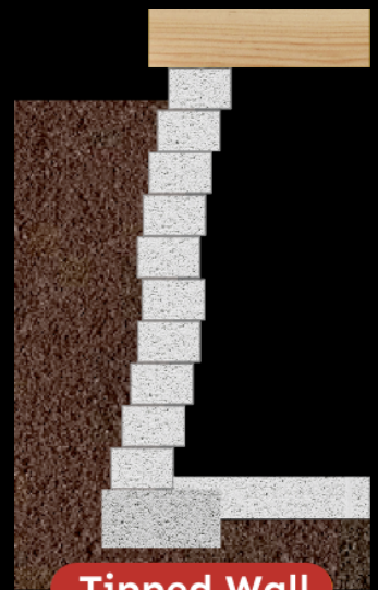
Tipped Wall
